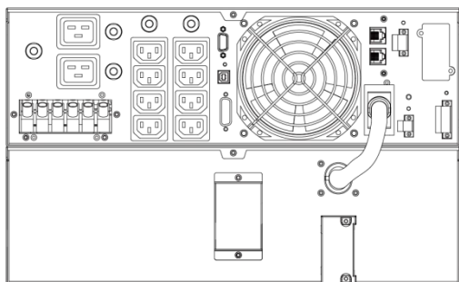
OL6000KERT3UPM
